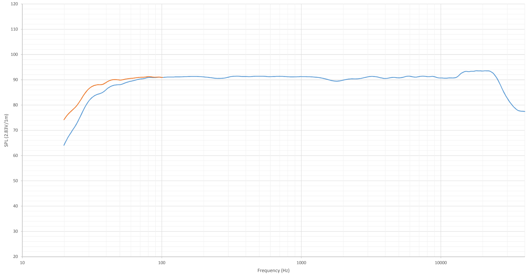
Frequency Response - Airmotiv T2
