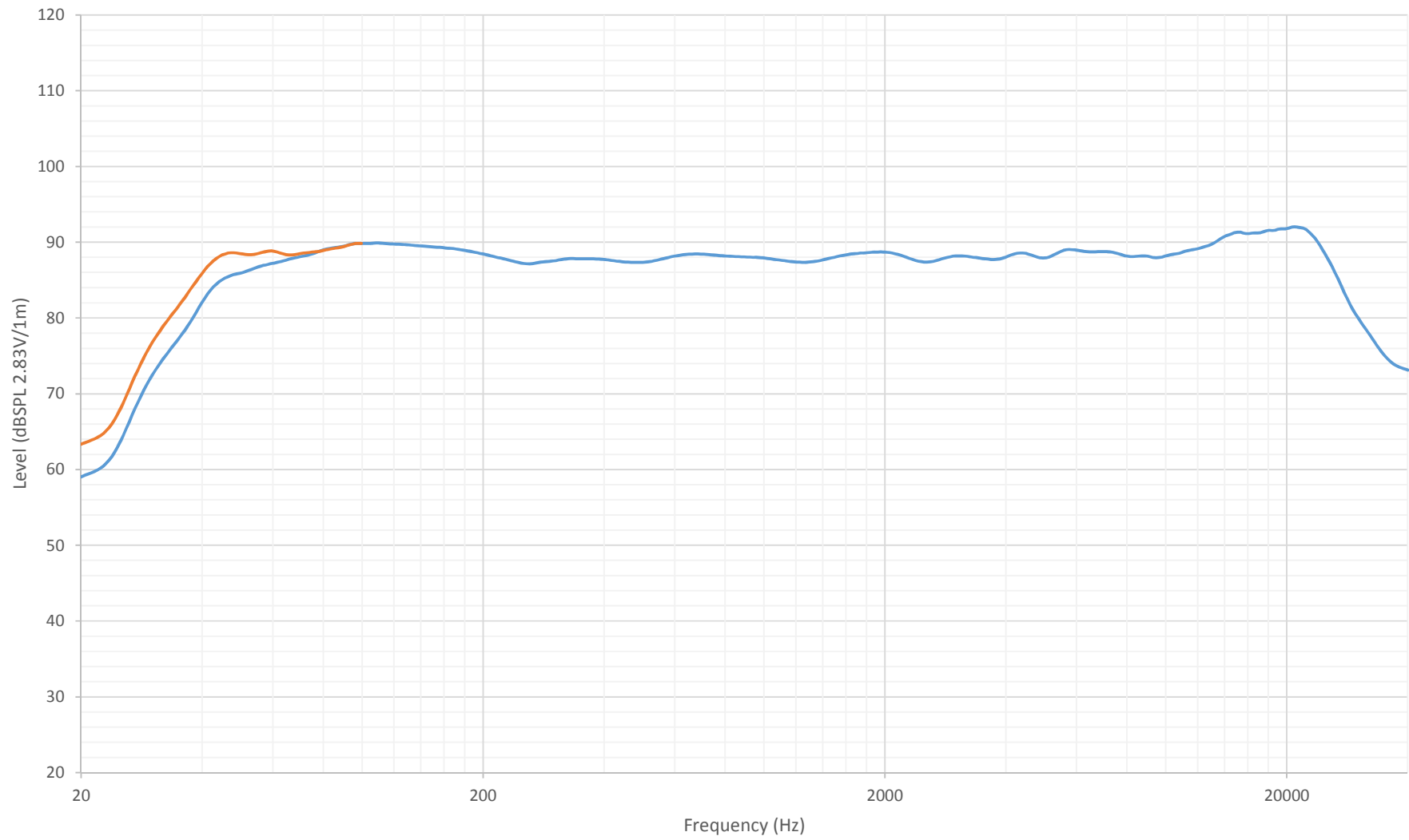
Frequency Response - Airmotiv T1
