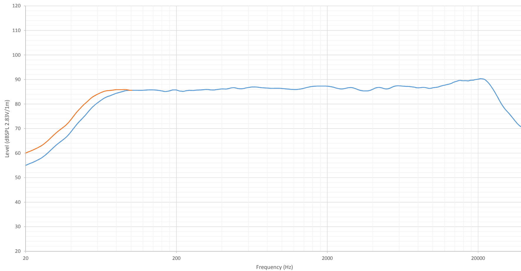
Frequency Response - Airmotiv B1
